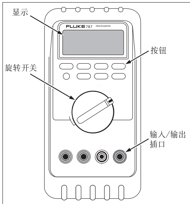
图 1. Fluke 787 ProcessMeter
