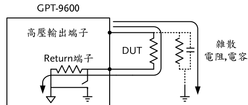
GROUND MODE = OFF, DUT floating
