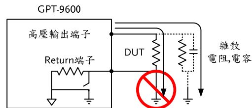
GROUND MODE = OFF, DUT grounded
