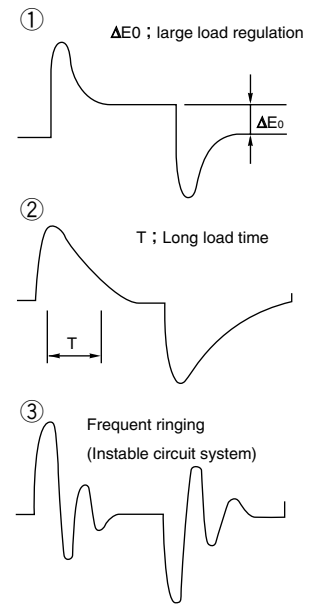
[Fig.-7 ] Transient Response Waveform
