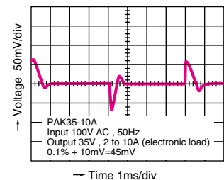
[Fig.-7 ] Transient Response Waveform
