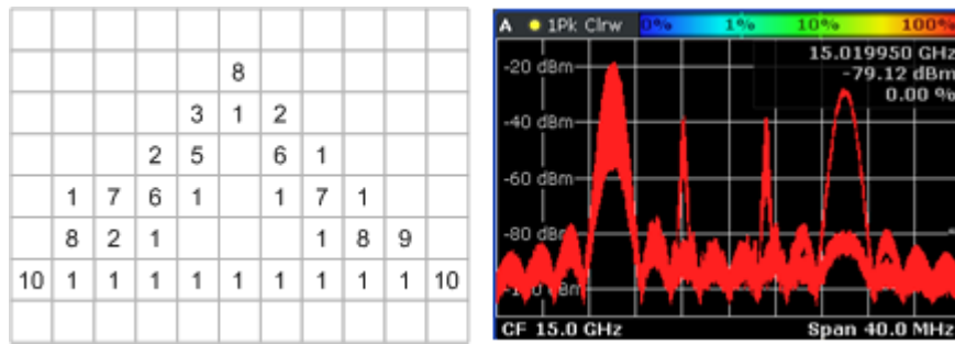
Figure 3-6: Virtual table and diagram containing the results after one frame (n FFTs)
