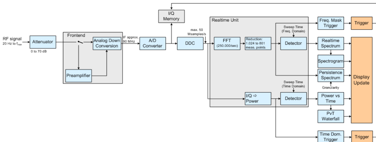
Figure 4-2: Block diagram of the R&S ESR
